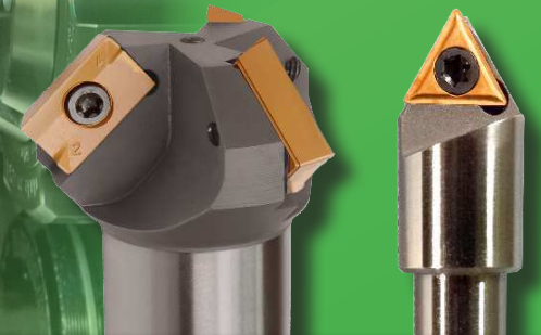
ROTATING TOOLS
