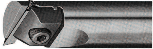
EVEREDE® Production Boring Bars are especially designed for Turret Lathes, and incorporate an adjusting screw behind the tool bit for quicker, fine adjustments.
