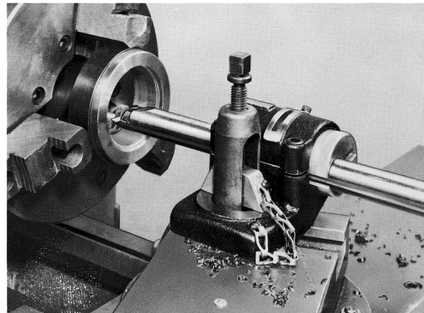
ENGINE LATHE
