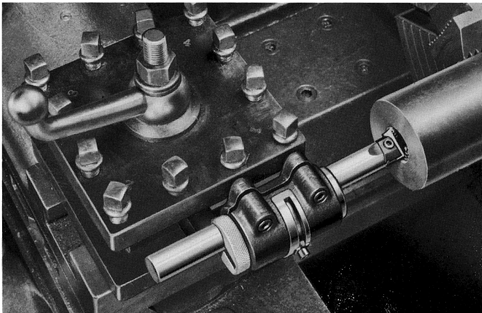
TURRET LATHE
